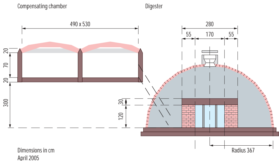
Cross-section of a 100-m 3 biodigester module
